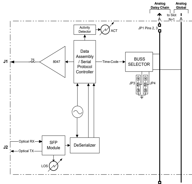
Figure 1: Module 9200-9181 Functional Diagram
