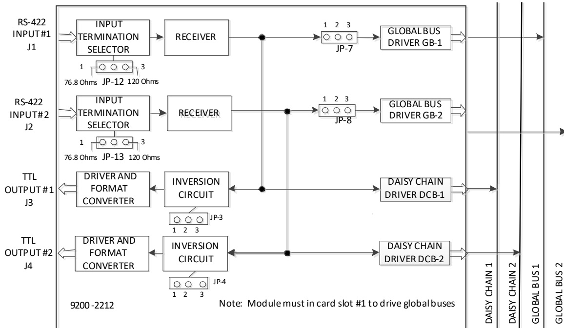
Figure 1: 9200-2212 Module Functional Drawing
